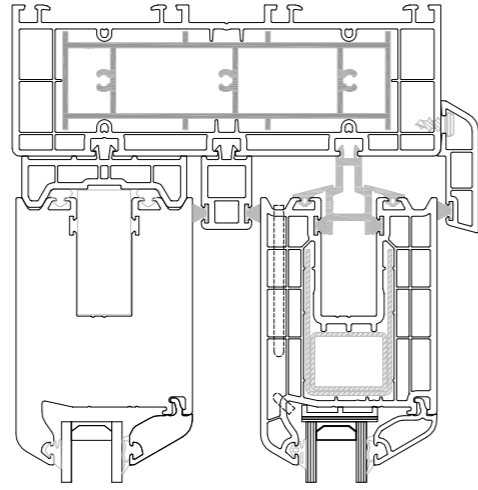
B-DETAYI
